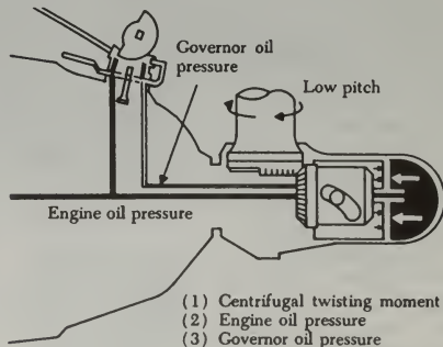
FIGURE 7-18. Diagram of hydromatic propeller operational forces.
